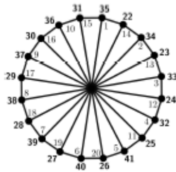
Figure 1: (22, 1) -distance antimagic labeling of Circ(20, \{1, 10\})
