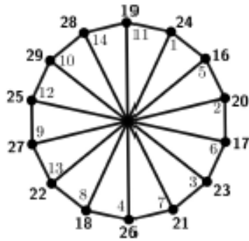
Figure 3: (16, 1) -distance antimagic labeling of Circ(14, \{1, 7\})
